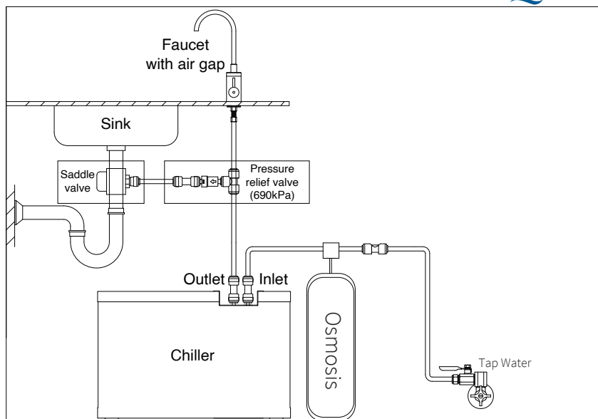
Image 2. Installation illustration
